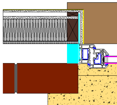
Typical new build jamb detail.
