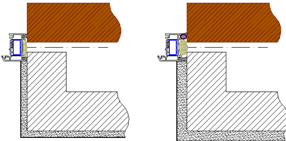
Flush reveal with joint width less than 6.0mm, frame bridging the DPM.
