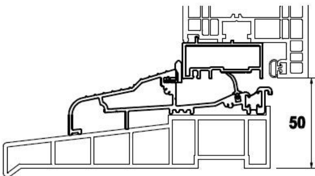
Open In Low Threshold On Cill
