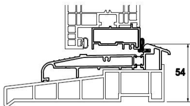
Open Out Low Threshold On Cill
