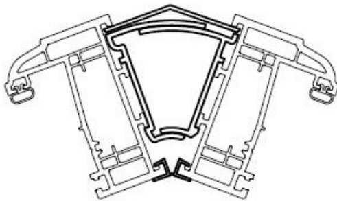
30° to 60° Variable Angle Post
