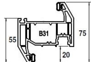
Externally Glazed Casement Sash
