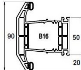
90mm Transom & Mullion
