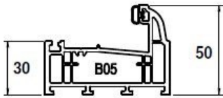
50mm Small Outer & Reduced Threshold
