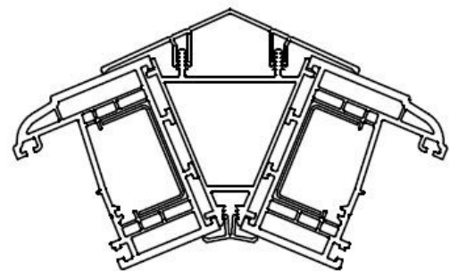
FLAT FIXED ANGLE BAY POST 135°
