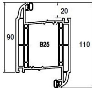
110mm Midrail & Mullion
