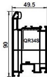
QC34 DEEP BOTTOM RAIL
