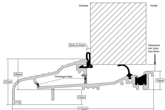
AM3 Open In Low Threshold On Cill
