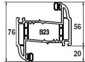
76mm Transom & Mullion
