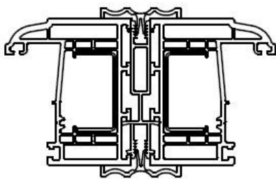
FLUTED COUPLING SECTION
