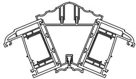
FLUTED FIXED ANGLE BAY POST 135°
