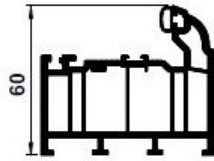
QS02 OUTER FRAME
