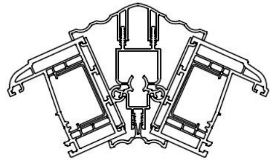
FLUTED VARIABLE POST 120° - 170°
