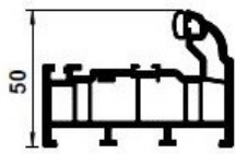
QS01 OUTER FRAME
