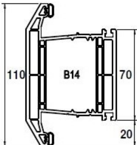
110mm Midrail & Mullion
