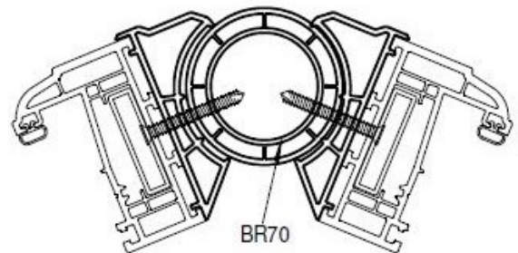
BR70 Round Bay Pole Assembly Overlapping
