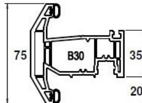
Internally Glazed Casement Sash
