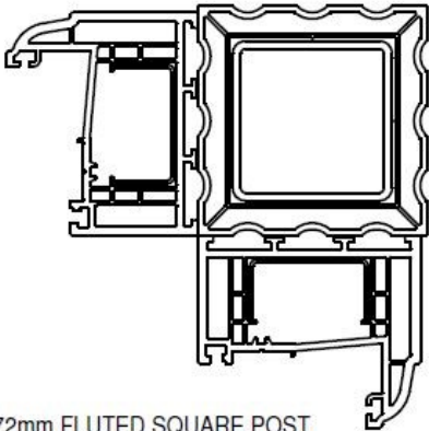
72mm FLUTED SQUARE POST
