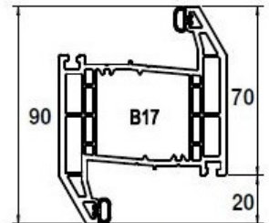
90mm Transom & Mullion
