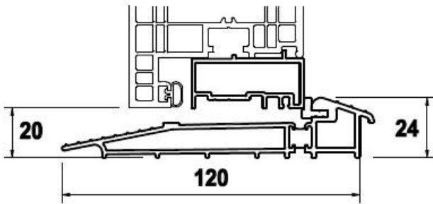
Open Out Low Threshold
