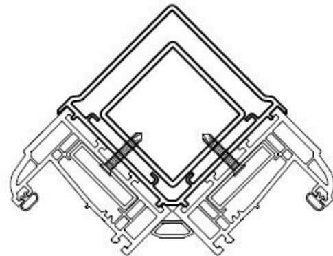
90° Bay Pole Overlapping
