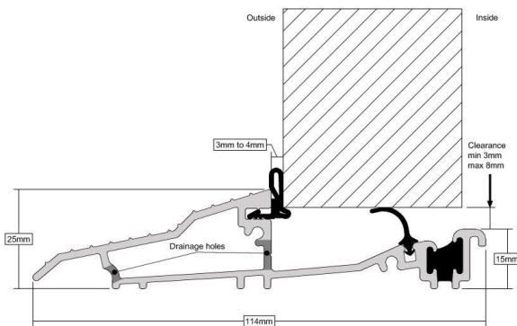
AM3 Open In Low Threshold
