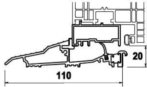
Open In Low Threshold
