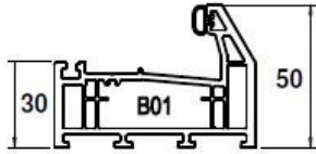
50mm Small Outer & Reduced Threshold
