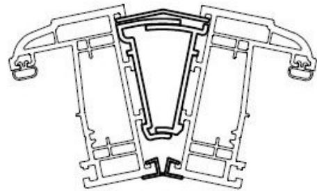
15° to 30° Variable Angle Post
